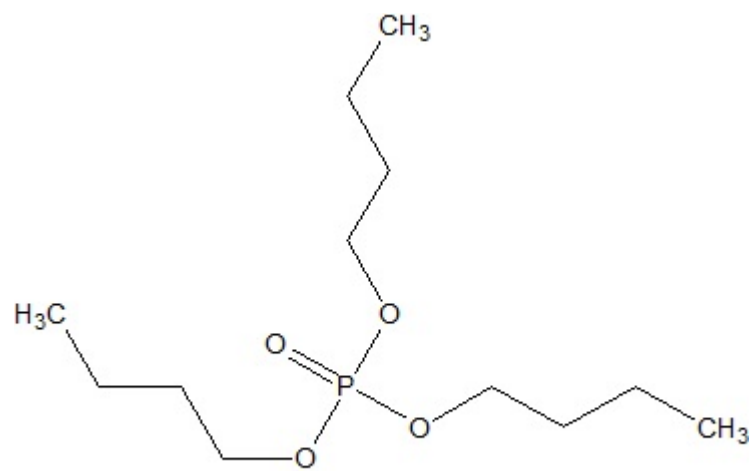
Tributyl Phosphate
